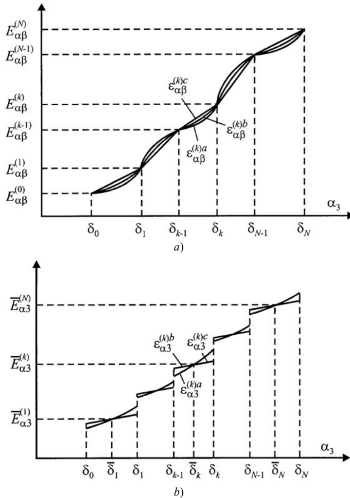
Fig. 3 Distribution of tangential (a) and transverse shear (b) strains over the shell thickness
